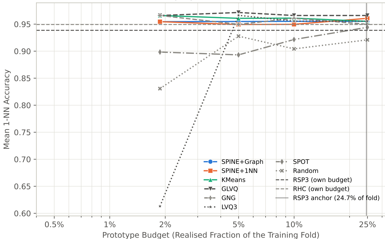
Accuracy against Budget - wine
