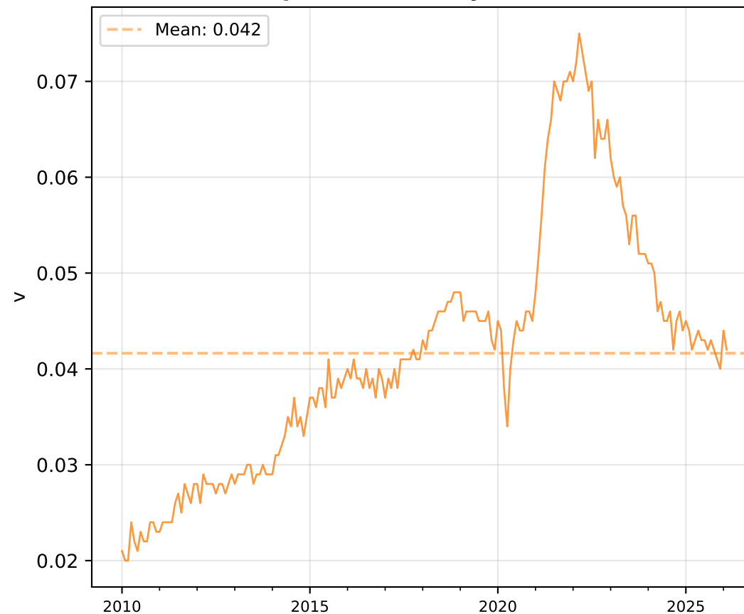
Simulated (Baseline): Vacancy Rate v(t)
