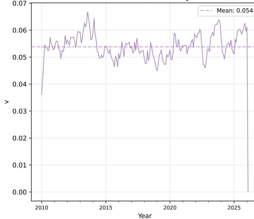
Simulated (Baseline): Vacancy Rate v(t)
