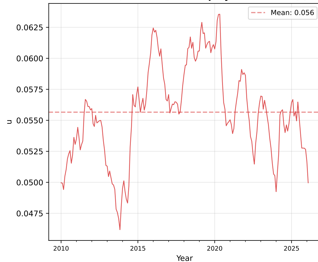
Simulated (Baseline): Unemployment Rate u(t)
