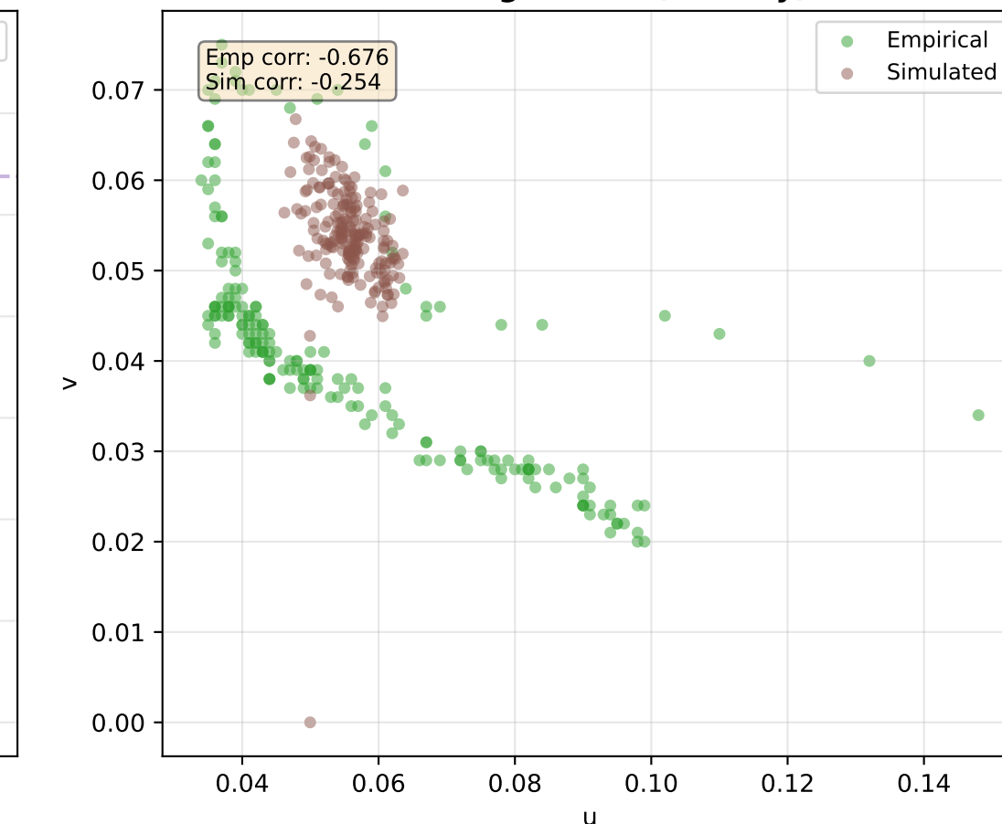
Beveridge Curve (Overlay)
