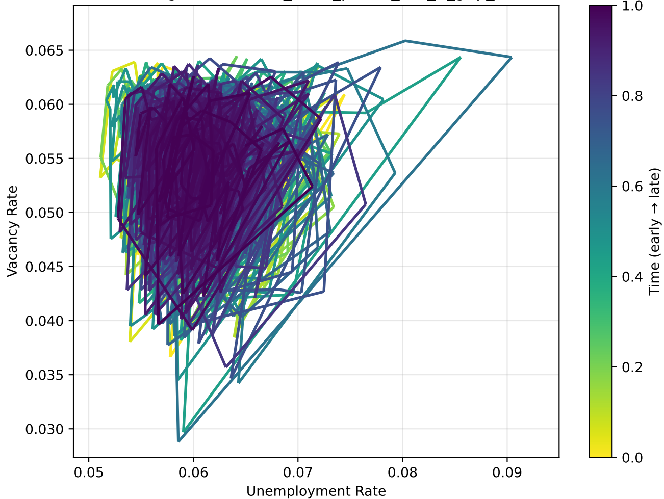
Beveridge Curve (250_firms_power_law_C_gdp_ar2)
