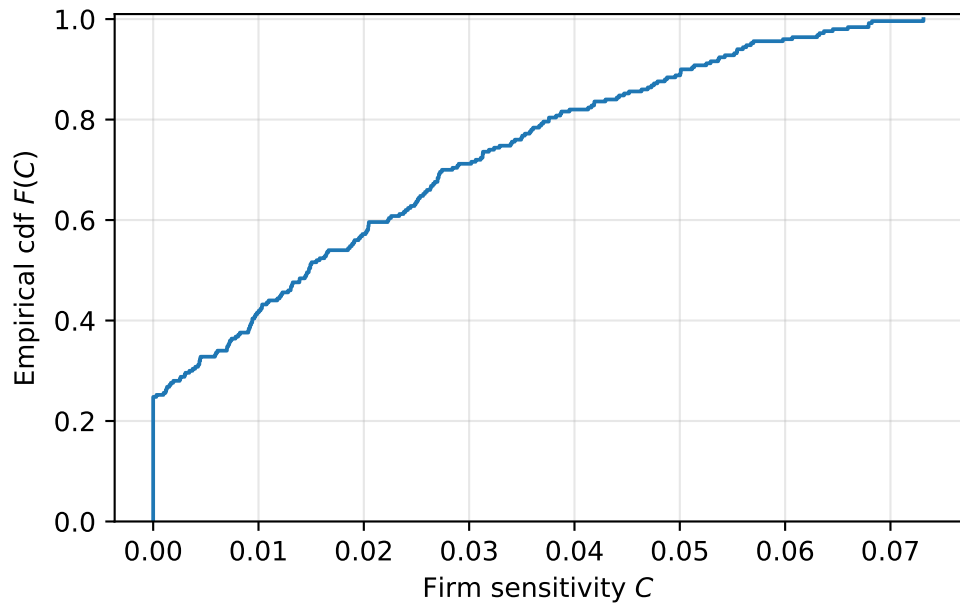
CDF
