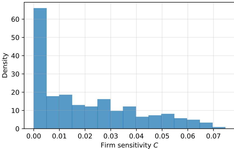
Histogram (normalized)
