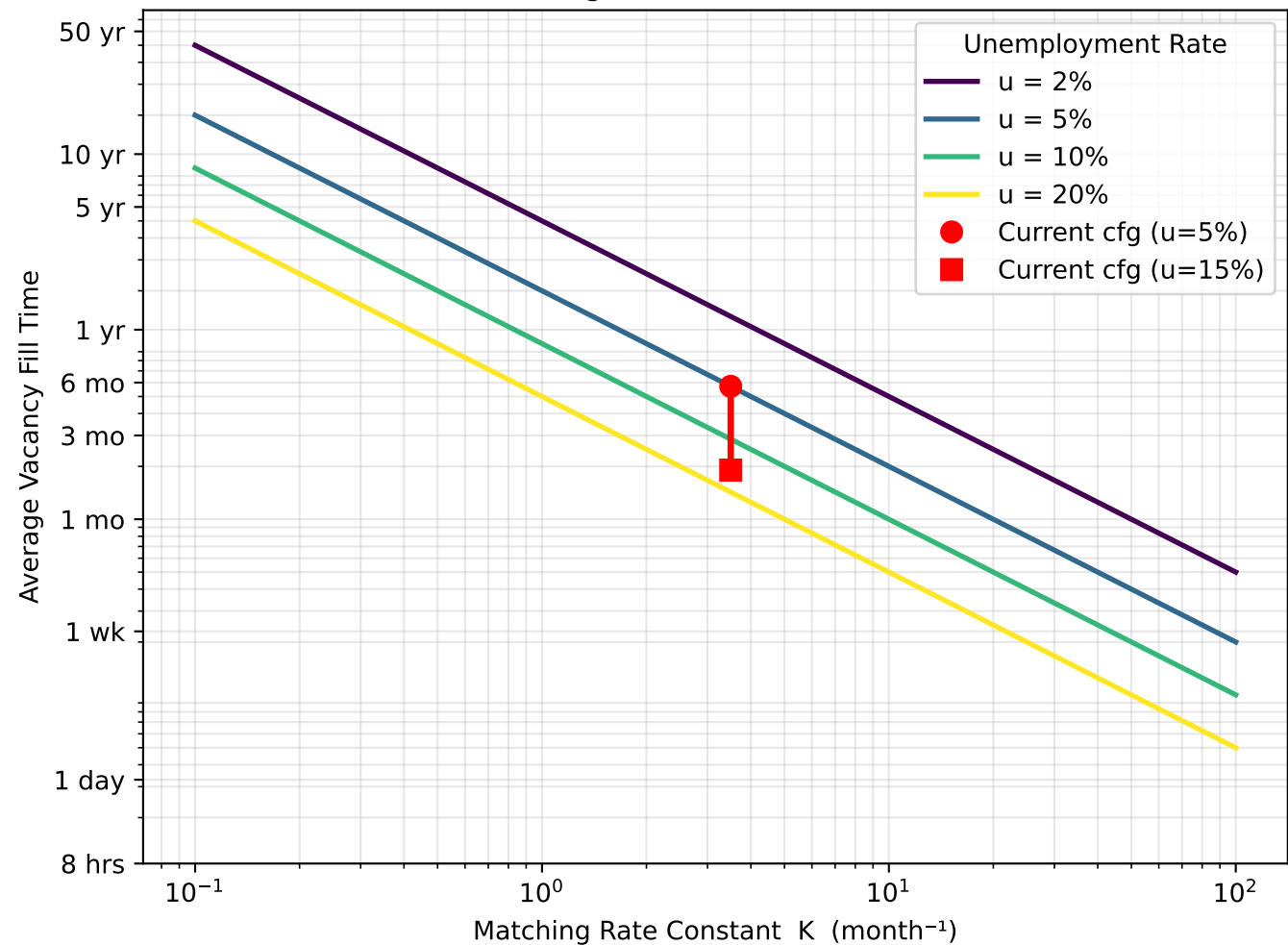
Matching Time \tau = 1/(K \cdot u) vs K
