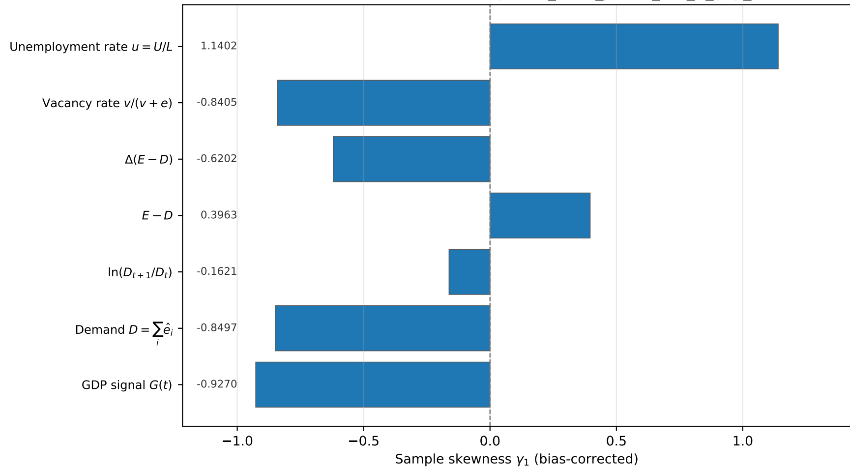
Post-burn-in skewness summary (250_firms_power_law_C_gdp_ar2)
