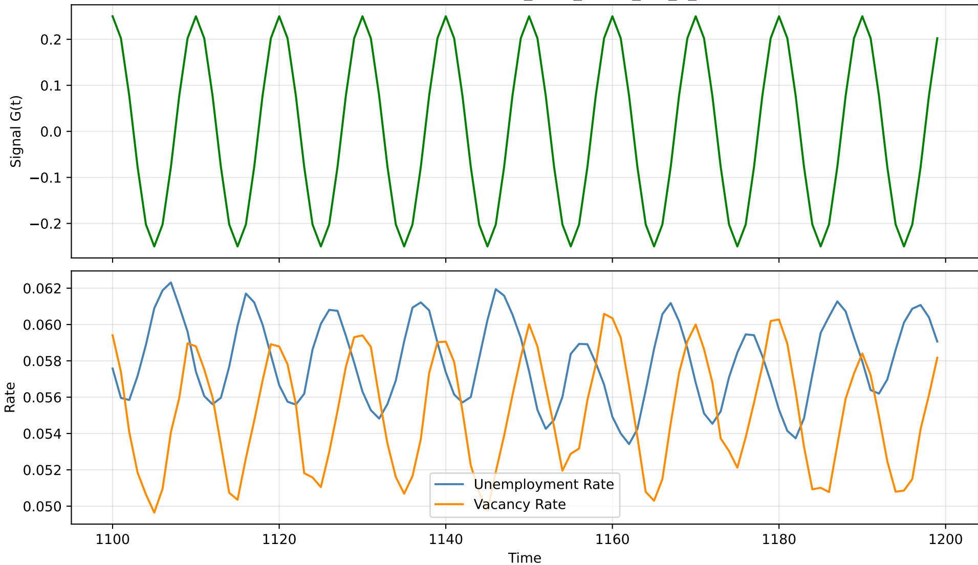
Aggregate Overview (250_firms_power_law_C_sine)
