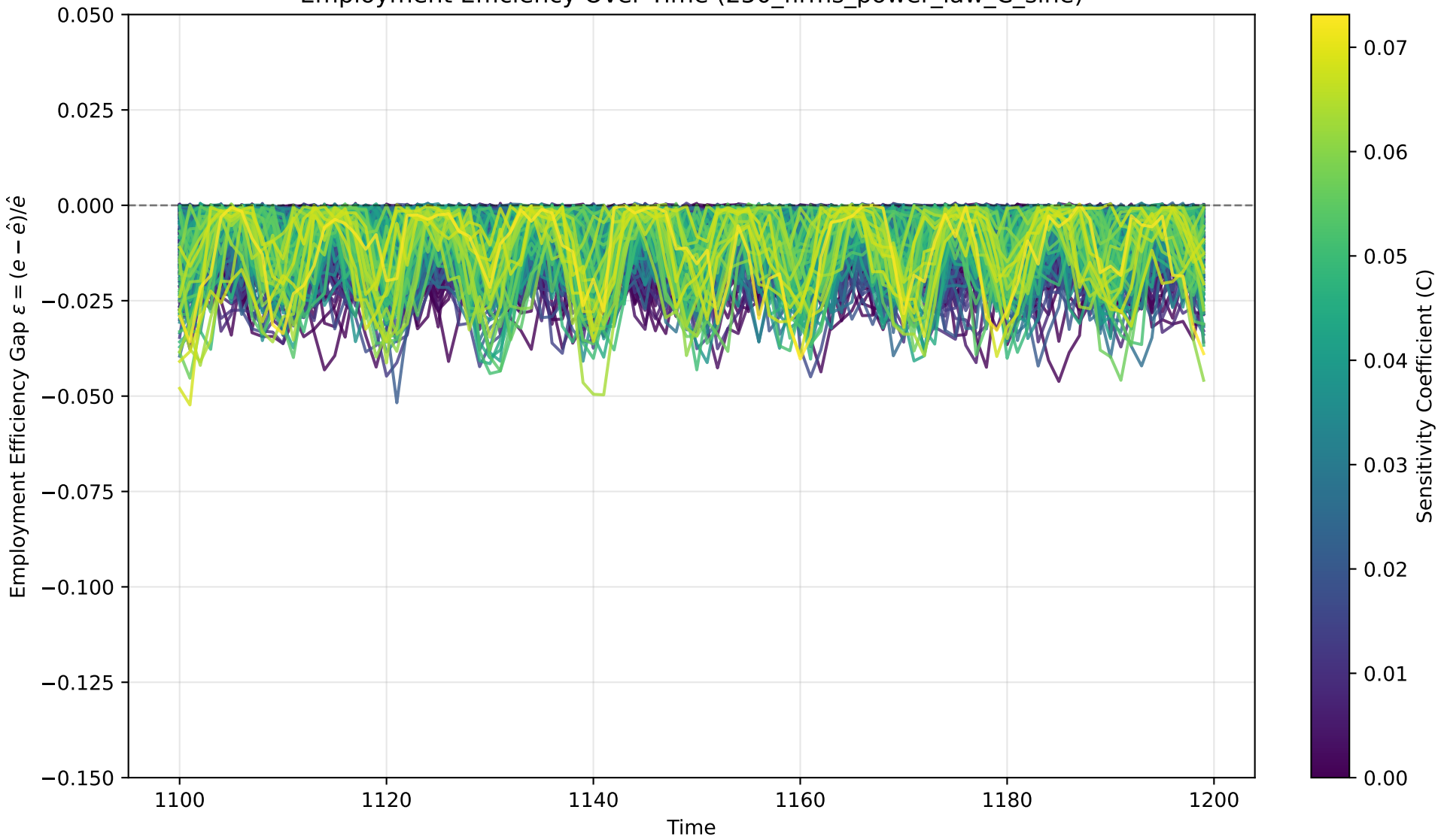
Employment Efficiency Over Time (250_firms_power_law_C_sine)
