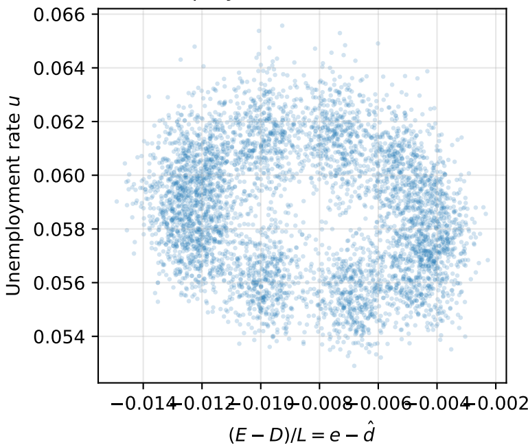
u vs employment – demand (rates)
