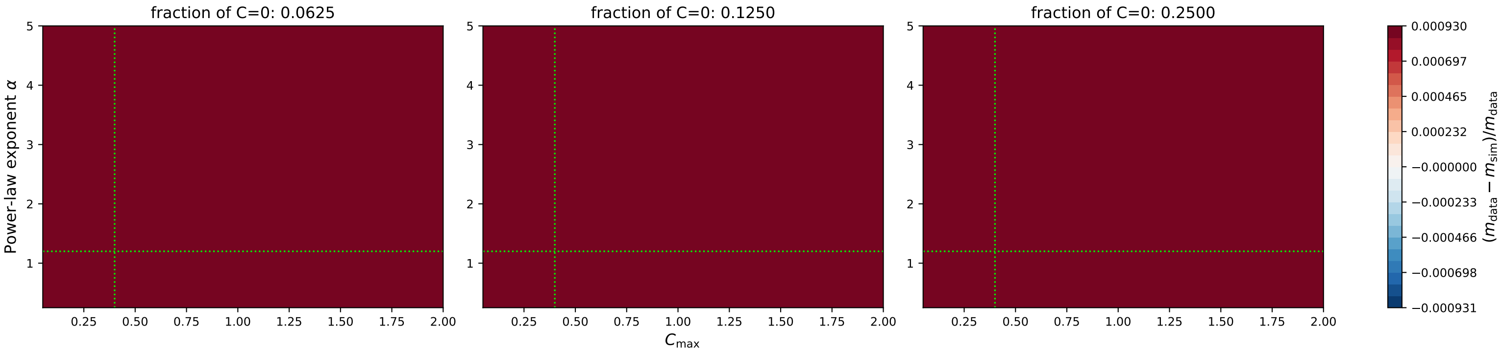
MSE vs empirical — Scan 1 — Normalised residuals ( m_{\text{data}} - m_{\text{sim}} )/ m_{\text{data}} ( C_{\text{max}} \times power-law exponent)
