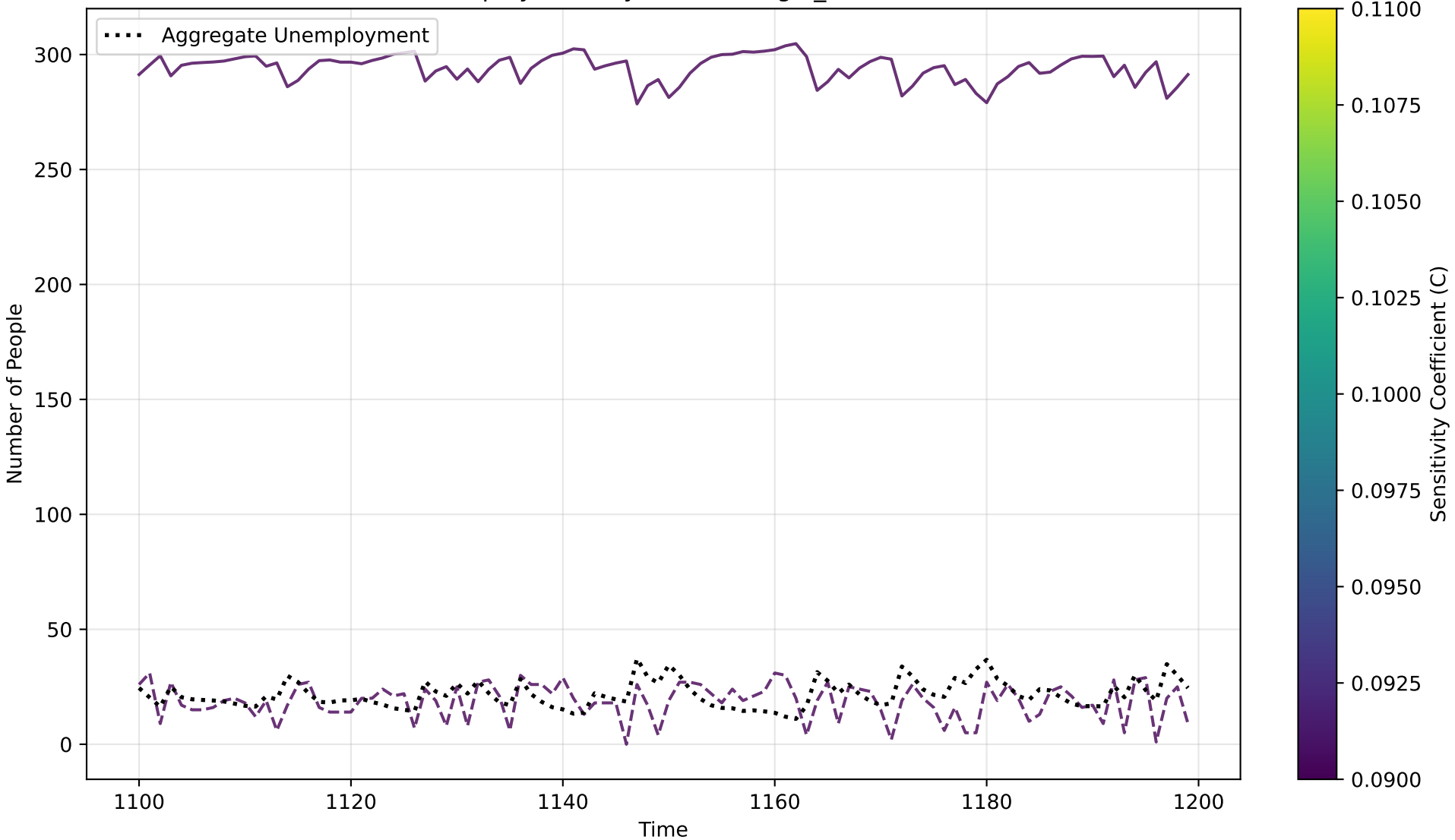
Employment Dynamics (single_firm)
