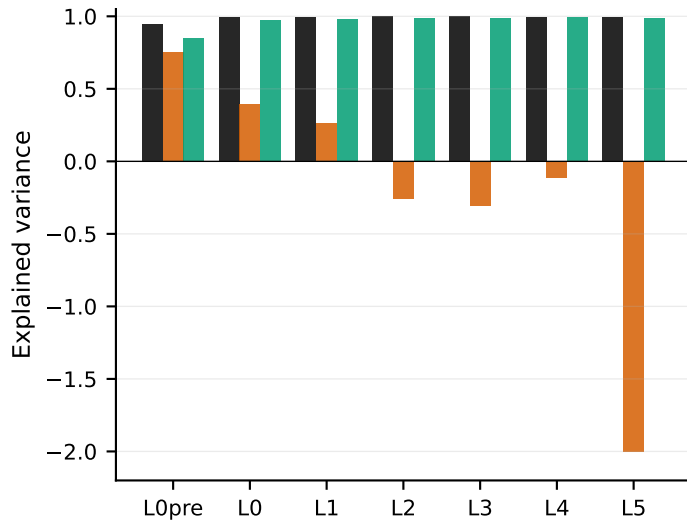
Pythia-70m (d_model = 512, 9 independent seeds)
