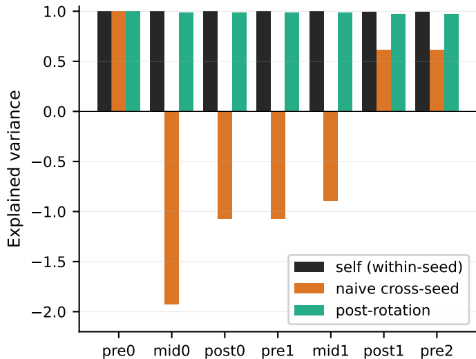
Dyck-3 toy (d_model = 64)
