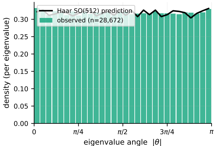
Eigenvalue spectrum of cross-seed R KS vs Haar: stat=0.0027, p=1.000
