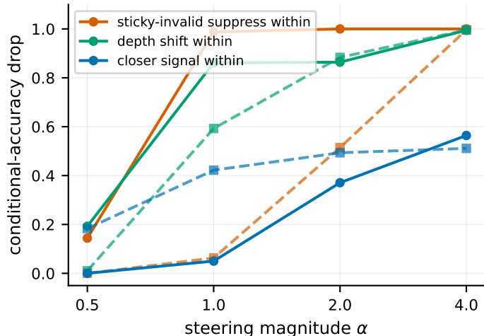
Dyck-3 (shared I/O): three regimes solid = within; dashed = cross-seed
