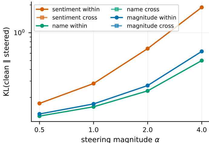
Pythia-70m (no shared I/O): all inverted solid = within; dashed = cross-seed
