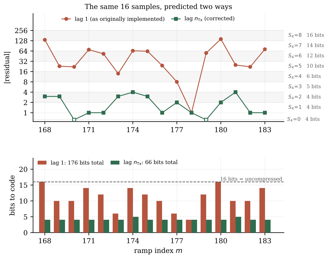
Figure 2: The 16-sample worked example plotted. Above: residual magnitude with the S4 cost bands marked. Below: bits per sample against the 16 uncompressed. 176 bits versus 66, for identical information.
