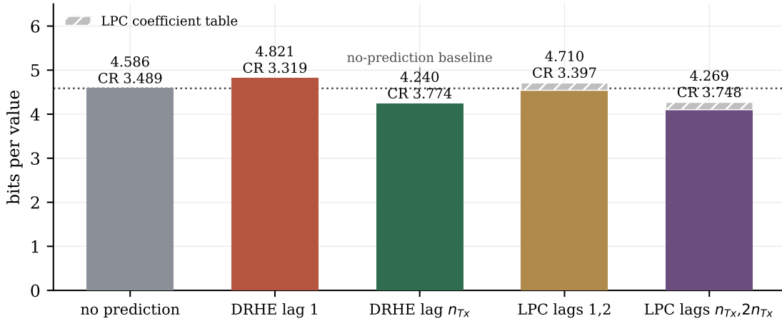
Figure 8.5: Bits per value for all five configurations, with the LPC coefficient table shown separately as it is charged whatever the residuals do. The dotted line is the no-prediction baseline: any bar above it is a predictor that is doing harm.
