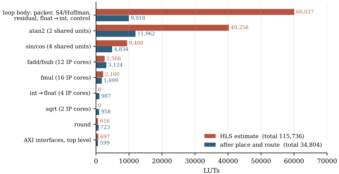
Figure 9.1: LUTs of each part of DRHE- n : the HLS estimate (from the module’s synthesis report) against the routed design (from the hierarchical utilisation report). The pre-built floating-point adders and multipliers were estimated well. The arctangent and the loop body, which HLS builds itself from C++, were over-estimated by factors of about three and six. The square root and the integer-to-float conversions were not estimated at all.
