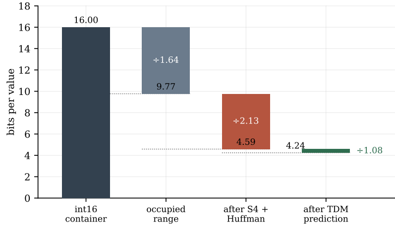
Figure 8.1: Where the compression ratio comes from. Of the 16 bits in the int16 container, 6.2 are structurally unused because the capture sits far below full scale; the entropy coder recovers a further factor of 2.13 from spectral sparsity; and prediction on the corrected axis contributes the remaining 1.08. Prediction on the original ramp axis contributes nothing at all — it costs 0.24 bits per value.
