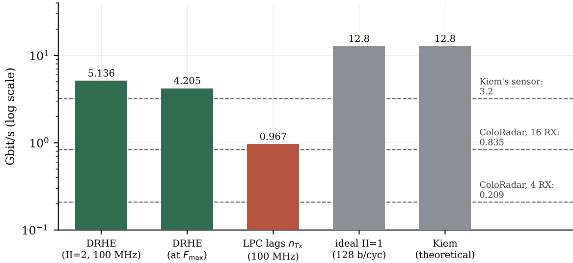
Figure 9.5: Throughput capacity (bars) against three requirements (dashed). Capacity above a dashed line is headroom. DRHE clears every requirement, including Kiem’s much faster sensor. The corrected LPC, measured over a whole frame, clears ColoRadar’s full 16-channel rate only narrowly, which matters only if frames arrive back-to-back.
