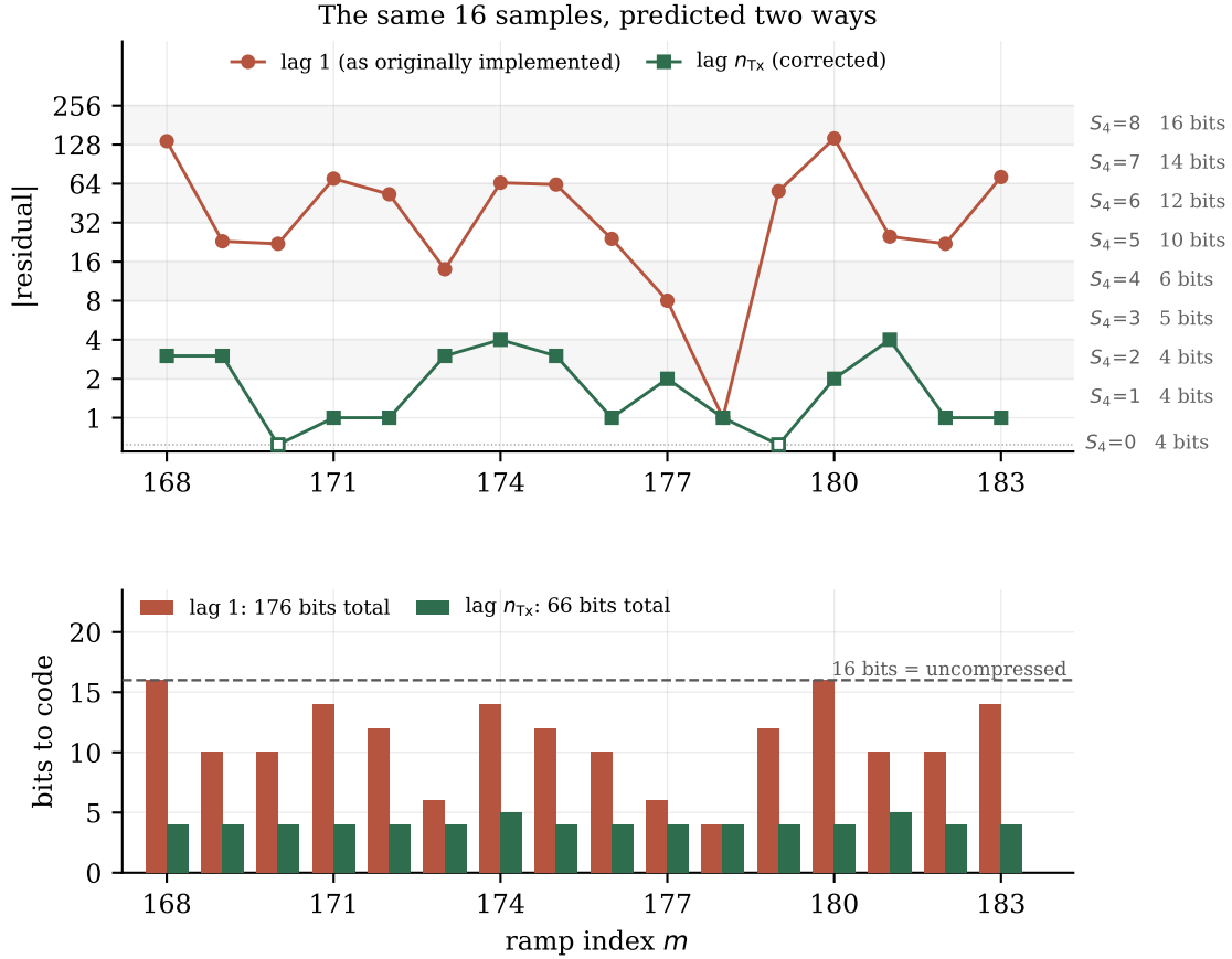
Figure 5.1: Table 5.4 drawn. Above: residual magnitude on a logarithmic scale, with the S_4 category bands and their bit costs marked on the right; hollow markers are residuals of exactly zero. Below: the bits each sample costs, against the 16 bits it would have taken uncompressed. The lag-1 predictor spends 176 bits on this window; the same predictor on the correct axis spends 66.
