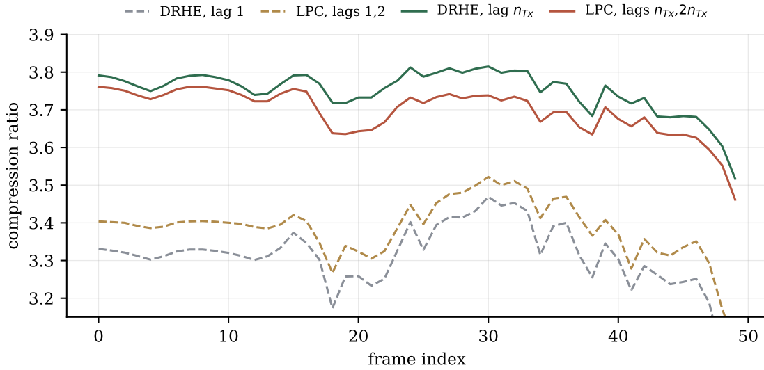
Figure 8.6: Per-frame compression ratio across the 50-frame sequence, measured in C-simulation. The corrected designs (solid) sit above their baselines on every frame, not merely on average, and the frame-to-frame variation — which tracks scene content — is preserved. All four configurations reconstruct every sample exactly.
