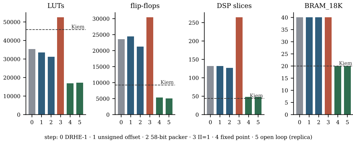
Figure 9.2: LUTs, flip-flops, DSPs and block RAM at each step of Table 9.5, all post-route on the xcku5p. The dashed line in each panel is Kiem’s published figure. Every step but one reduces the design; the exception raises it from II = 2 to II = 1, which doubles the arithmetic because the units can no longer be shared between channels.
