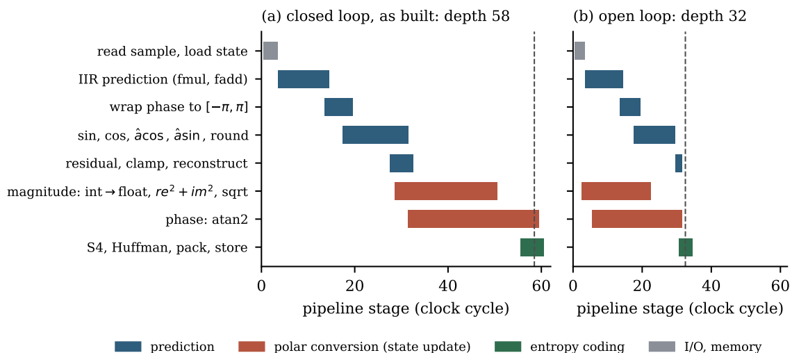
Figure 9.3: The pipeline schedule of one sample, read from the HLS schedule reports. (a) DRHE-1 as built: the state is updated from the reconstructed sample, so the polar conversion (red) waits for the prediction (blue) and the depth is 58. (b) The same float design with the state updated from the input sample (open loop): the two chains run side by side and the depth is 32. Kiem’s design is open loop and fixed point, and shorter still.
