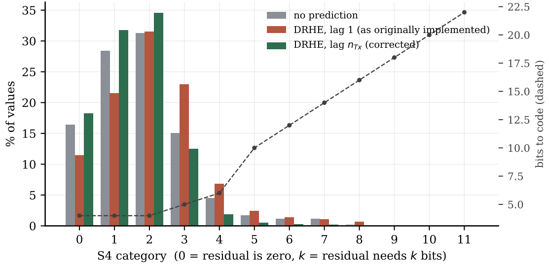
Figure 8.3: Distribution of residuals across S_4 categories, with the cost of each category (Equation (5.7)) on the right axis. Lag-1 DRHE (red) pushes mass up the category scale relative to not predicting at all (grey) — into categories 3 and 4 which cost 5 and 6 bits. Lag- n_{Tx} DRHE (green) pulls it back down into categories 0–2, which cost 4 bits or fewer. The steepness of the cost curve above category 4 is what makes this shift so consequential.
