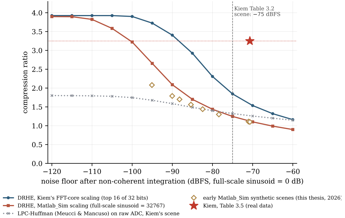
Figure 10.2: Compression ratio against noise floor on Kiem's Table 3.2 scene with one transmitter. Blue: DRHE with Kiem's fixed dictionary and his FFT core's scaling. Red: the same with the Matlab_Sim scaling, four times larger. Grey: LPC-Huffman of [27] on raw ADC. Diamonds: the early synthetic scenes of this thesis. Star: Kiem's published 3.25 at −70.7 dBFS, which lies 17 dB to the right of where his own scaling's curve passes 3.25.
