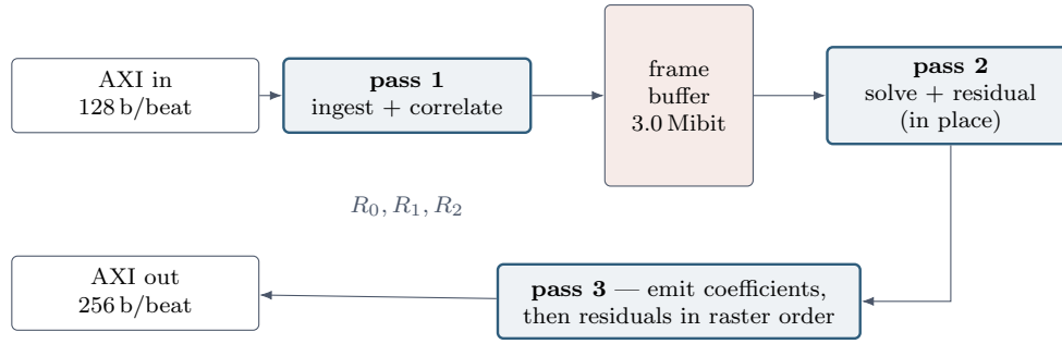
Figure 7.1: The LPC compressor. Because the Yule–Walker coefficients depend on the whole frame, the compressor must buffer it; the buffer is then rewritten in place with residuals so that only one memory is needed. Emitting residuals in the original raster order is what lets the decompressor avoid a frame buffer entirely.
