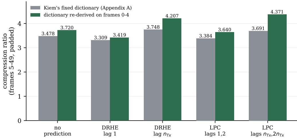
Figure 8.8: Compression ratio on held-out frames 5–49 with Kiem’s fixed dictionary and with a dictionary re-derived from frames 0–4. The gain is 3–8 % for the raw codes and the uncorrected predictors and 12–18 % for the corrected ones, and with the re-derived dictionary LPC overtakes DRHE.
