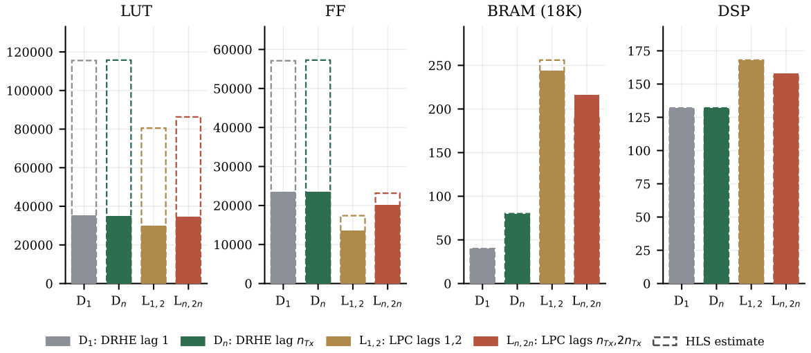
Figure 8.7: Resource usage for the four designs, post-route (solid) against the HLS estimate (dashed outline). Once implemented the four designs use similar logic; they differ in memory. The TDM correction moves DRHE’s BRAM from 40 to 80 and, by removing the ingest accumulators, moves LPC’s down .
