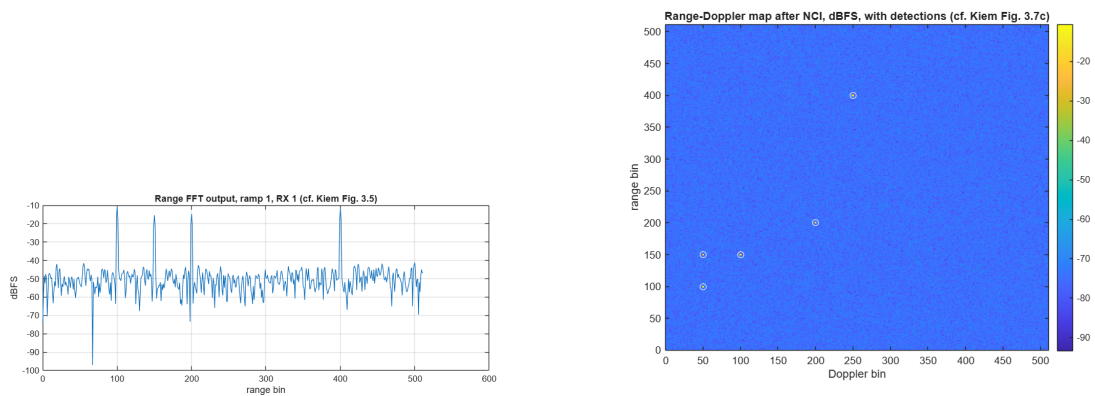
Figure 10.1: Kiem's Table 3.2 scene as rebuilt. Left: range FFT of ramp 1, receiver 1 (compare his Figure 3.5). Right: range-Doppler map after NCI with the five reference detections circled (compare his Figure 3.7c).
