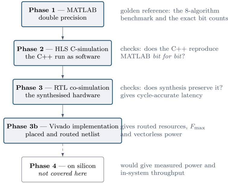
Figure 6.1: The verification ladder. Each phase is checked against the one above it, so a mismatch localises to a single transition rather than to “somewhere in the design”.
