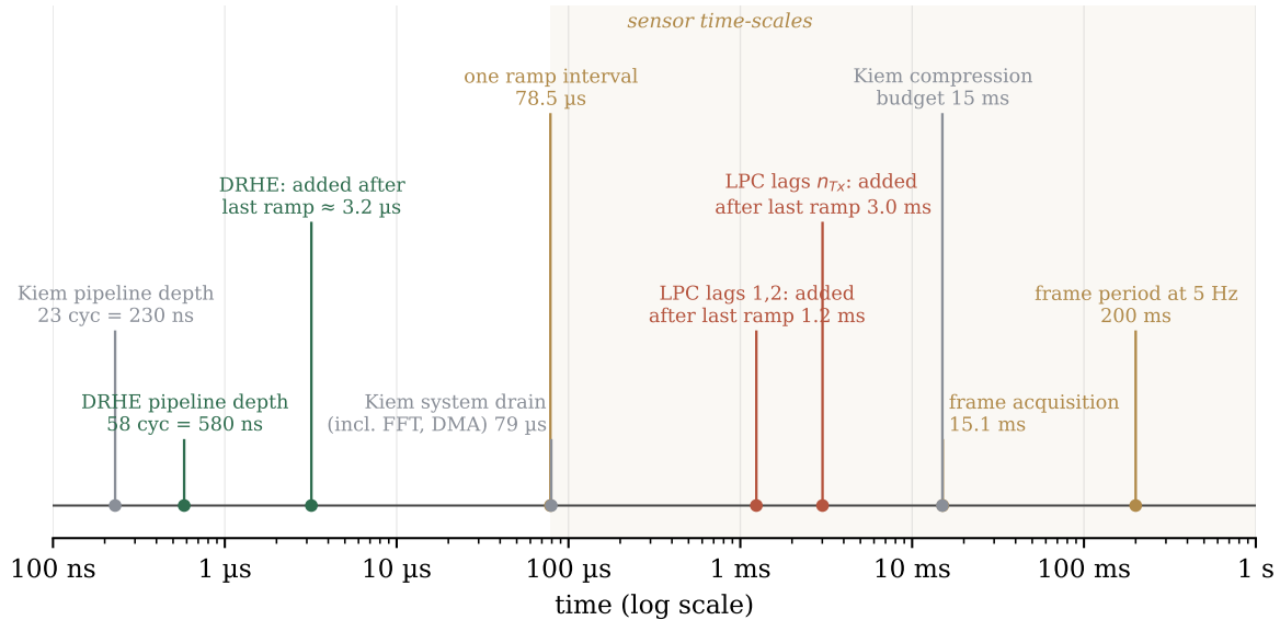
Figure 9.4: Every latency in this chapter on one logarithmic time axis. The compressor’s own delays (left) are two to five orders of magnitude shorter than the sensor’s time-scales (shaded). The only compressor delays that approach the sensor’s scale are LPC’s, because LPC must see the whole frame before it can emit anything.
