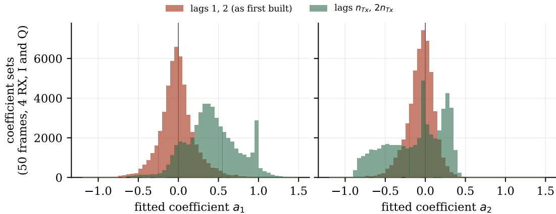
Figure 8.2: Distribution of the fitted, quantised LPC coefficients over 50 frames (51,200 sets). On the transmitter-interleaved axis (lags 1, 2, red) the fit drives both coefficients towards zero — the predictor nearly switches itself off. On the true slow-time axis (lags n_{Tx} , 2n_{Tx} , green) a_1 moves to a median of 0.40, with a cluster near 1 from bins containing strong, slowly changing returns. Computed by the independent implementation of Appendix D.
