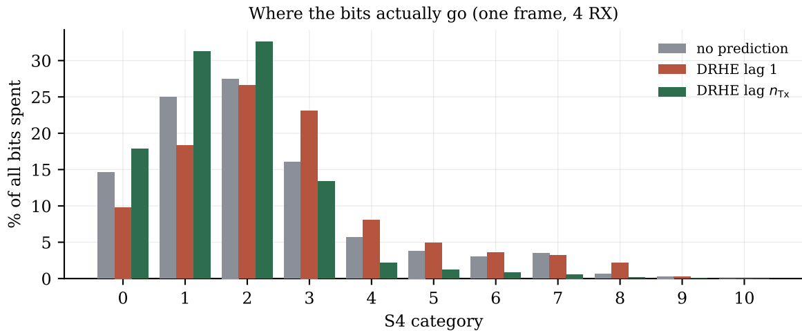
Figure 5.2: The “% bits” columns of Table 5.6 drawn. The corrected predictor concentrates spending into the three four-bit categories; the lag-1 predictor pushes it out into categories 3 through 8, where each value costs two to four times as much.
