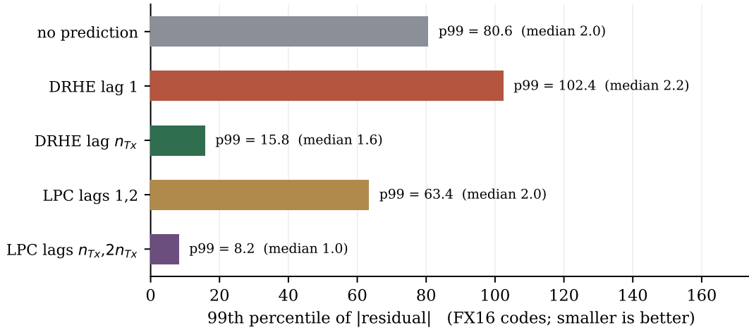
Figure 8.4: The 99th percentile of residual magnitude. This is the clearest single view of the effect: lag-1 DRHE produces a heavier tail than no prediction at all (102.4 against 80.6), while lag- n_{Tx} DRHE cuts it to 15.8 — a factor of 6.5 better than the design it replaces. LPC at lags n_{Tx}, 2n_{Tx} reaches 8.2.
