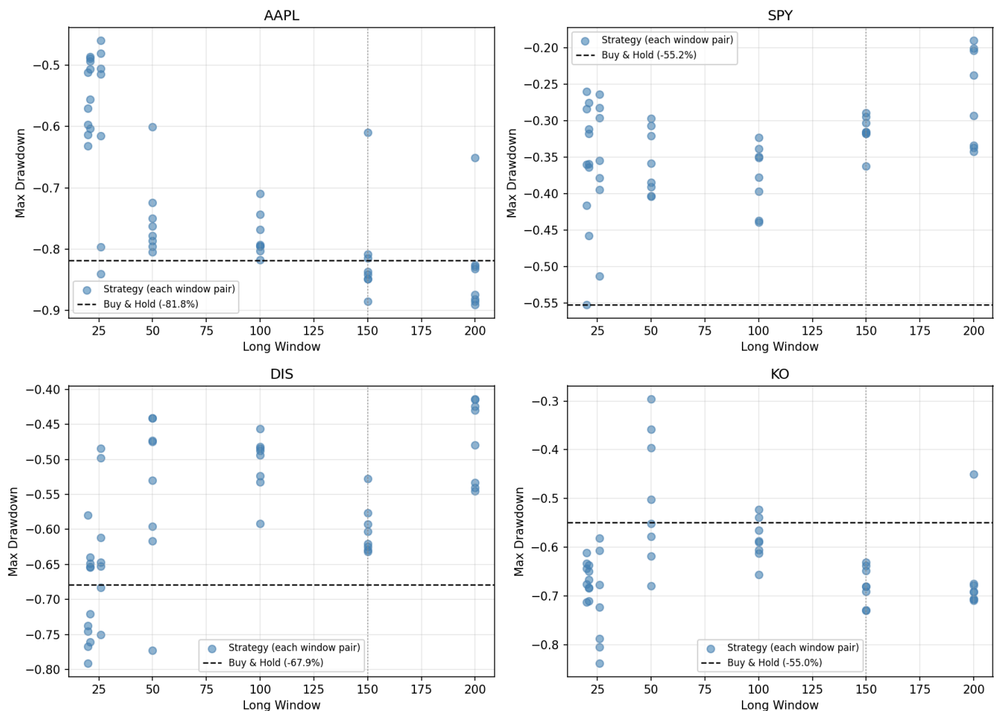
Max Drawdown vs Long Window, by Ticker (dashed line = Buy & Hold, dotted = 150-day mark)
