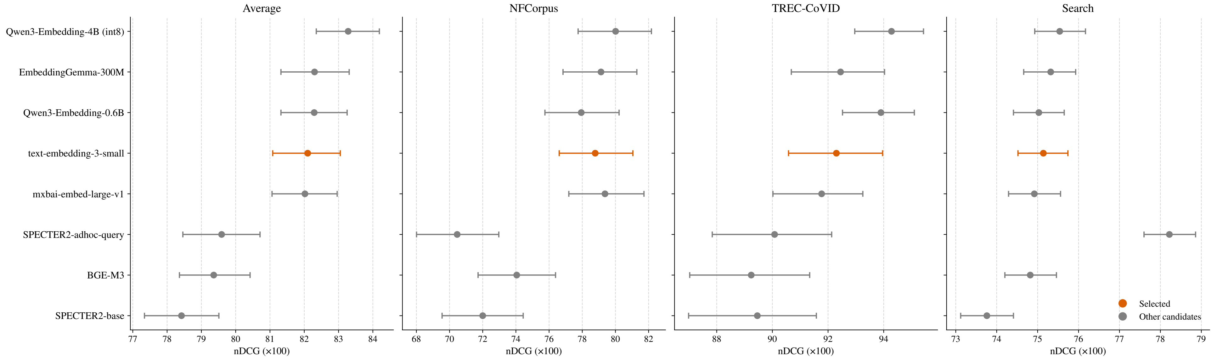
Dense bi-encoder nDCG: Average and per-dataset (model order fixed by Average), 95% bootstrap CIs
