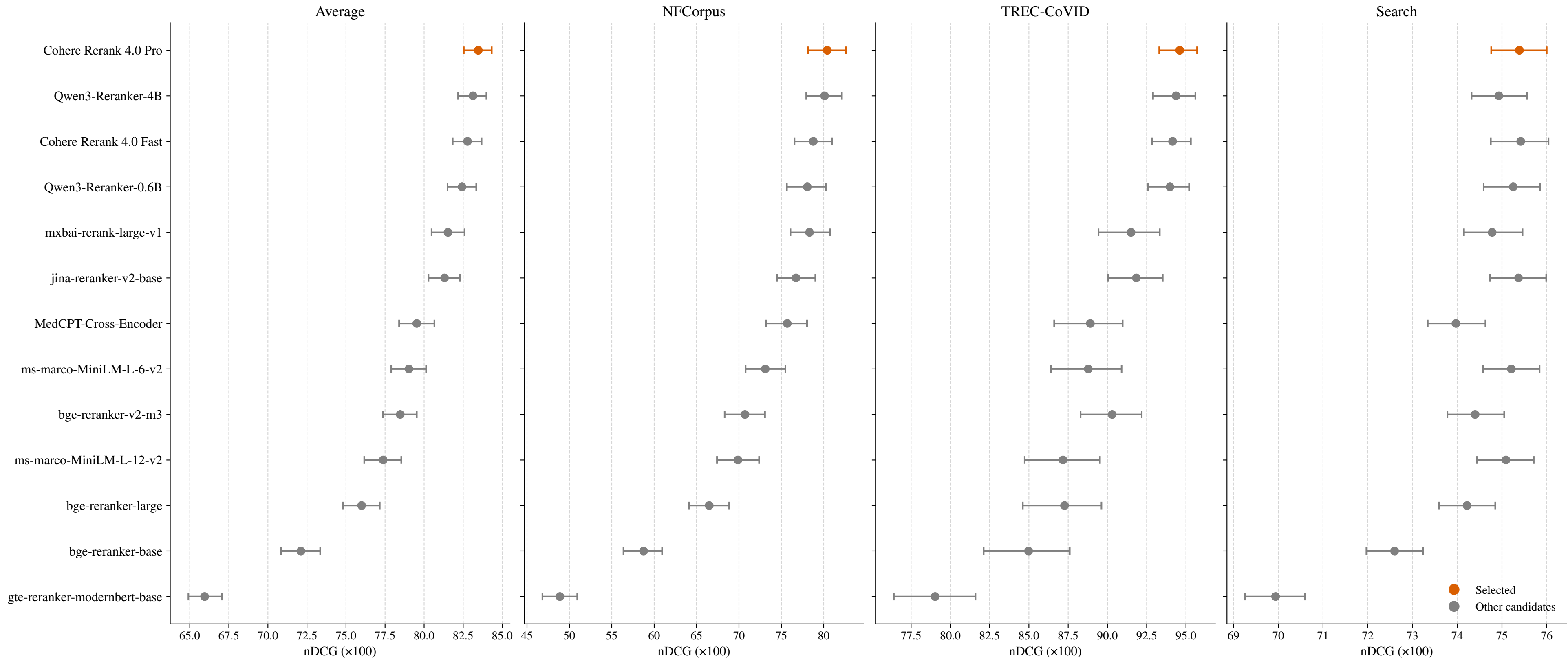
Cross-encoder nDCG: Average and per-dataset (model order fixed by Average), 95% bootstrap CIs
