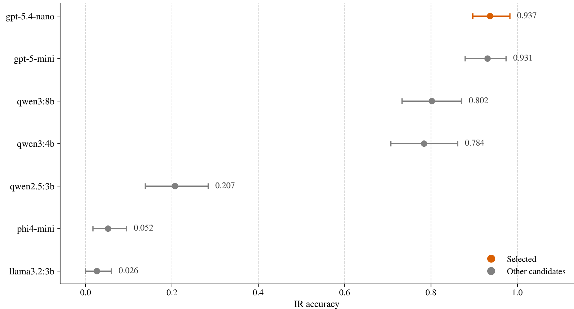
NL-to-IR accuracy by model, with 95% bootstrap CIs
