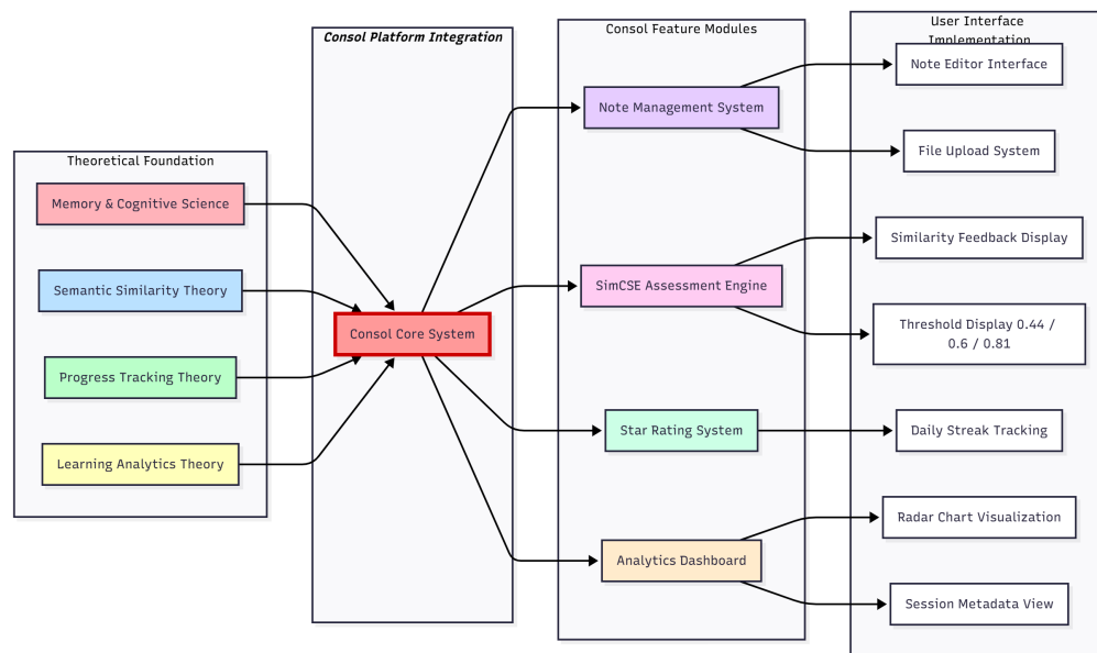
Figure 3.1: Comprehensive integrative framework showing the evolution from foundational research domains through Consol feature implementation to final platform integration. The diagram illustrates how theories from memory science, semantic similarity research, progress tracking, and learning analytics converge into Consol’s unified system.
