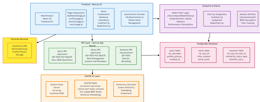
Figure 4.5: Comprehensive development architecture diagram detailing API endpoints, database schema relationships, and system component interactions. The diagram shows the technical infrastructure supporting educational assessment workflows including user management, content processing, and performance analytics.
