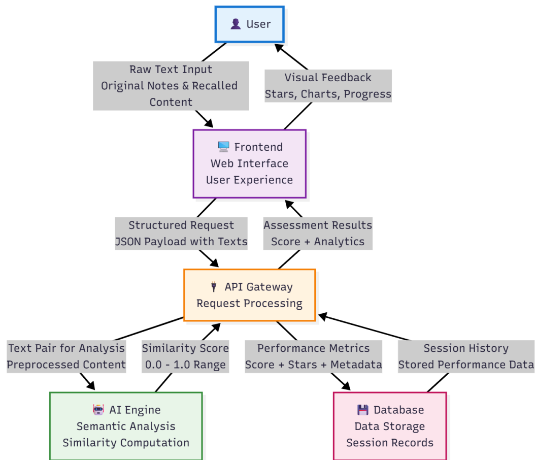
Figure 4.1: Basic system architecture showing the complete data flow cycle from user input through semantic processing to educational feedback. The diagram illustrates five core layers: User Interface, Frontend Web Application, API Gateway, AI Engine, and Database Storage, with labeled data transformations at each processing stage.
