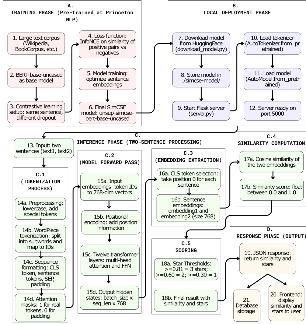
Figure 4.2: Comprehensive SimCSE architecture diagram showing the complete processing pipeline from input sentence tokenization through BERT encoding, contrastive learning mechanisms, and final similarity computation. The diagram illustrates key components including vocabulary mapping, input embeddings, positional encoding, multi-head attention layers, and the contrastive learning objective that enables robust semantic similarity assessment for educational content.
