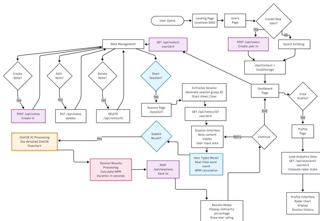
Figure 4.7: Comprehensive user interaction flow diagram showing the complete educational workflow including decision trees, session management processes, and iterative assessment cycles. The diagram illustrates user pathways from authentication through content creation, assessment sessions, and performance analysis.
