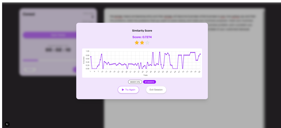
Figure 5.6: Session Score
