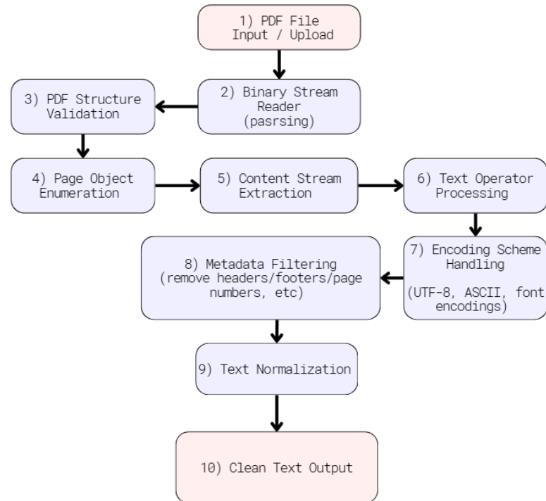
Figure 4.2: PDF document processing pipeline showing binary parsing, page object extraction, and text reconstruction for semantic similarity preparation.
