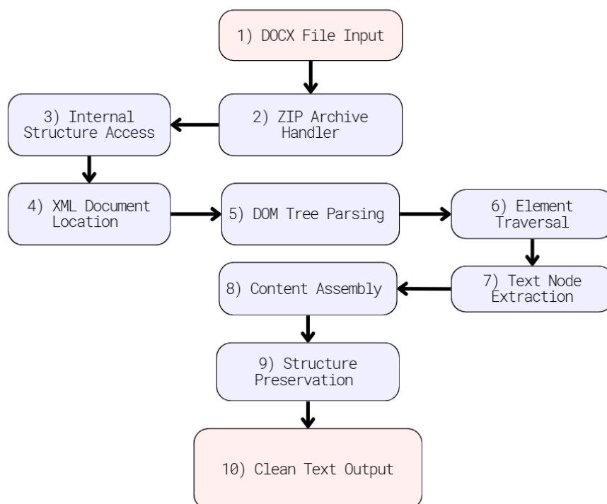
Figure 4.3: DOCX document processing pipeline illustrating ZIP extraction, XML parsing, and structured text assembly for semantic analysis preparation.
