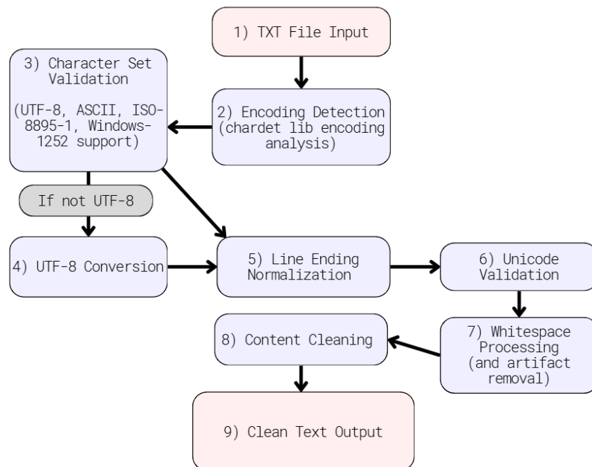
Figure 4.4: Plain text processing pipeline demonstrating encoding detection, UTF-8 normalization, and content validation for semantic similarity preparation.
