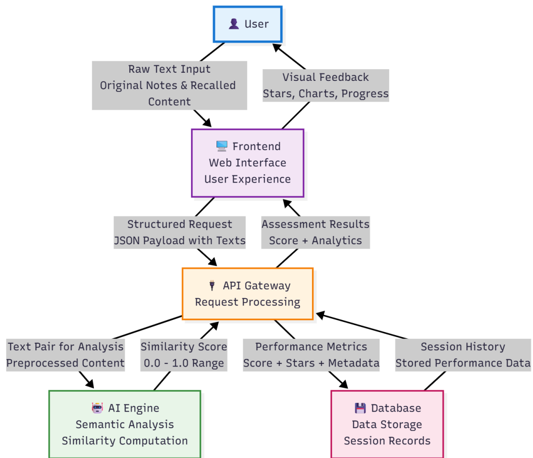
Figure 4.1: System architecture showing the complete data flow cycle from user input through semantic processing to feedback. The diagram illustrates four core components: Frontend Web Interface, API Gateway, AI Engine, and Database Storage, with labeled data transformations at each processing stage.
