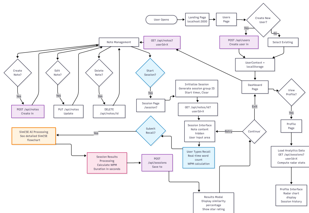
Figure 4.5: Comprehensive user interaction flow diagram showing the complete educational workflow including decision trees, session management processes, and iterative assessment cycles. The diagram illustrates user pathways from authentication through content creation, assessment sessions, and performance analysis.
