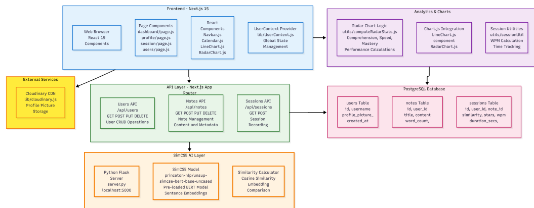
Figure 4.3: Comprehensive development architecture diagram detailing API endpoints, database schema relationships, and system component interactions. The diagram shows the technical infrastructure supporting educational assessment workflows including user management, content processing, and performance analytics.
