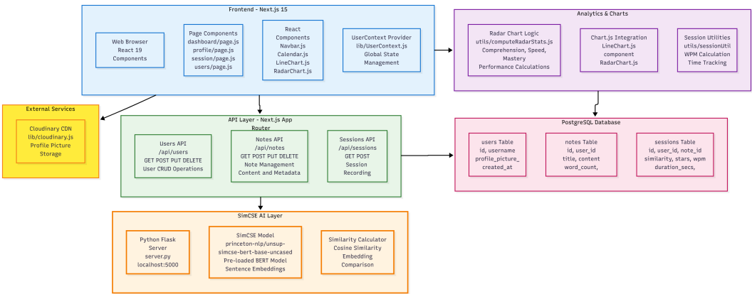
Figure 4.7: Development Architecture Diagram
