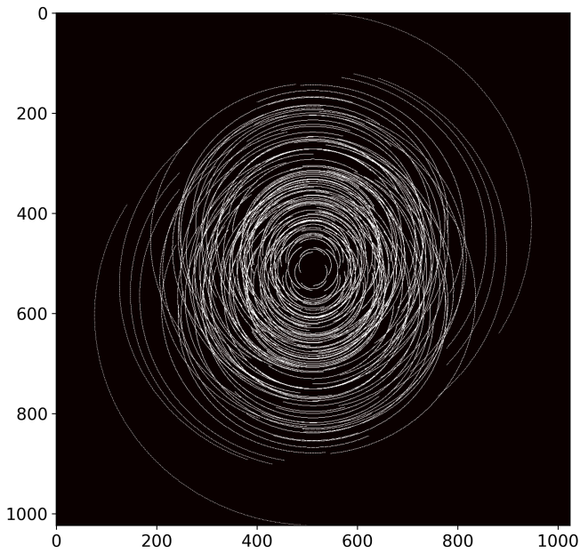
Fig. 6. High-resolution uv -coverage tracks generated by the optimal genetic algorithm layout. The hot colour map indicates sampled spatial frequency pixels, with brighter regions corresponding to denser baseline track overlap.
