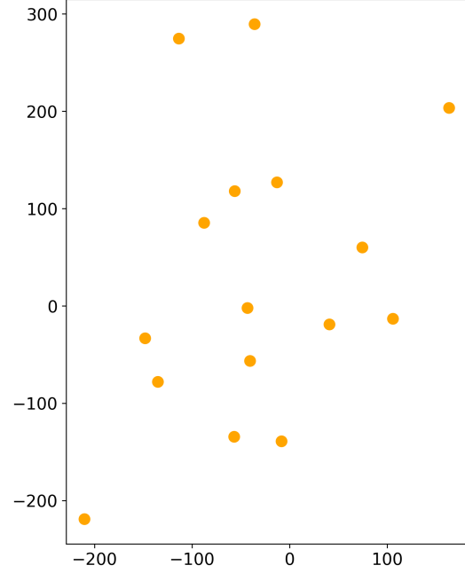
Fig. 7. Physical spatial layout of the optimal 16-antenna configuration discovered by simulated annealing. The pronounced central clustering of antenna positions is visually apparent relative to the more dispersed genetic algorithm solution.
