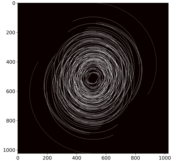
Fig. 8. High-resolution uv -coverage tracks generated by the optimal simulated annealing layout. The dense central sampling region reflects the short-baseline geometry of the clustered physical configuration.
