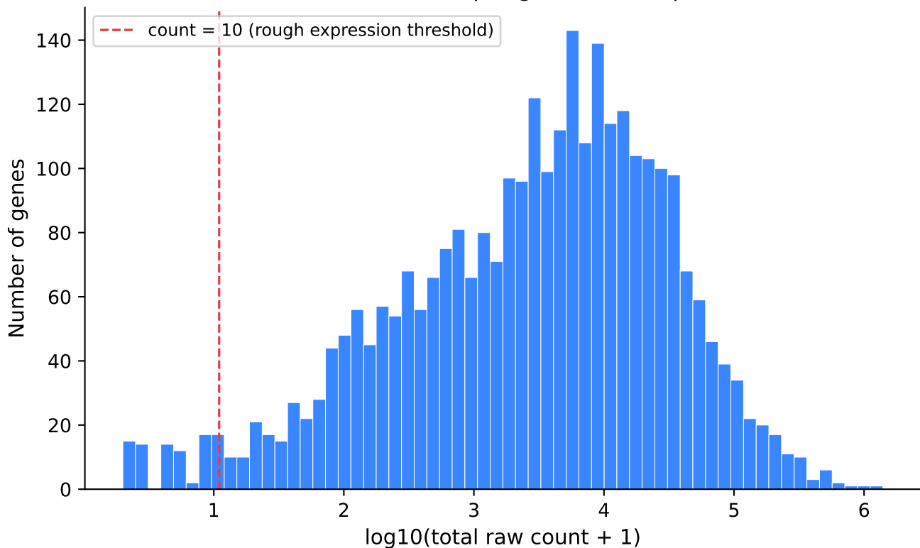
Distribution of raw counts per gene (all samples summed)
