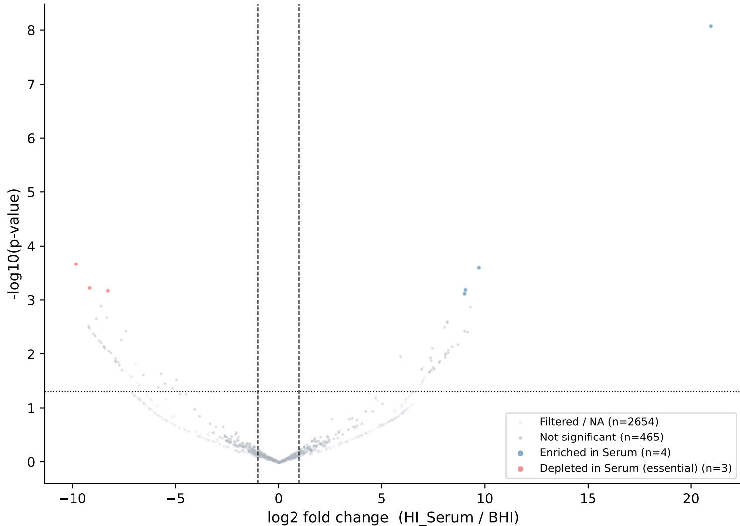
Tn-seq volcano: HI Serum vs BHI (sorted by padj)
