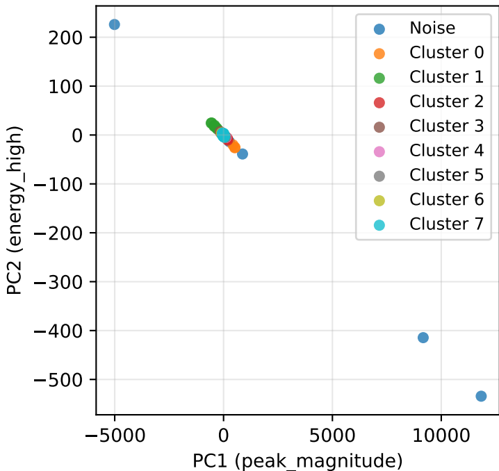
Binary Anomaly Clusters
