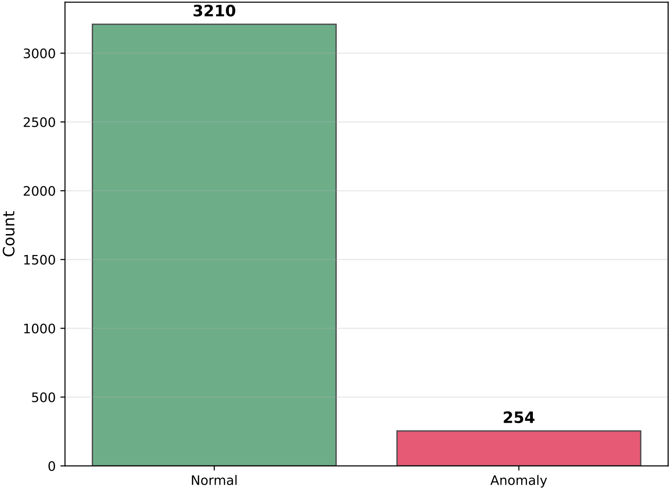
Detection Statistics
