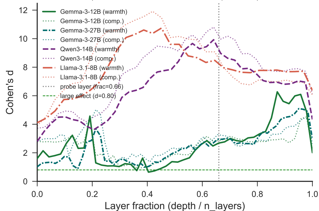
Representation strength by depth (solid = warmth, dotted = competence)
