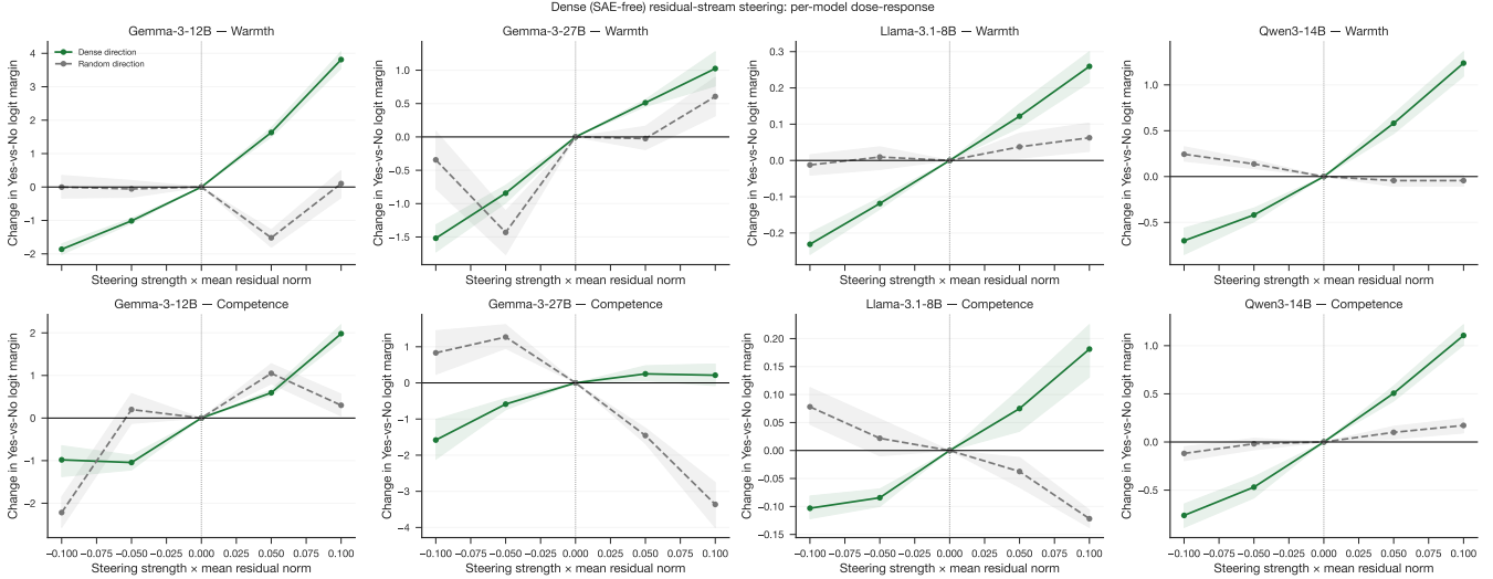
Figure 4: Concept-level steering dose-response curves. Mean logit-margin shift (Yes–No on warmth/competence judgements) as a function of steering strength \alpha (expressed as a fraction of the mean residual-stream norm) for the dense target direction across all four models. Positive slopes confirm that all models respond causally to the extracted direction vectors; the substantially higher slope at Gemma-3-12B (warmth slope = 27.79, R^2 = 0.956 ) compared to Gemma-3-27B (slope = 12.89, R^2 = 0.990 ) illustrates the steerability difference despite identical probe accuracy. Error bars are bootstrapped 95% confidence intervals over held-out topics.
