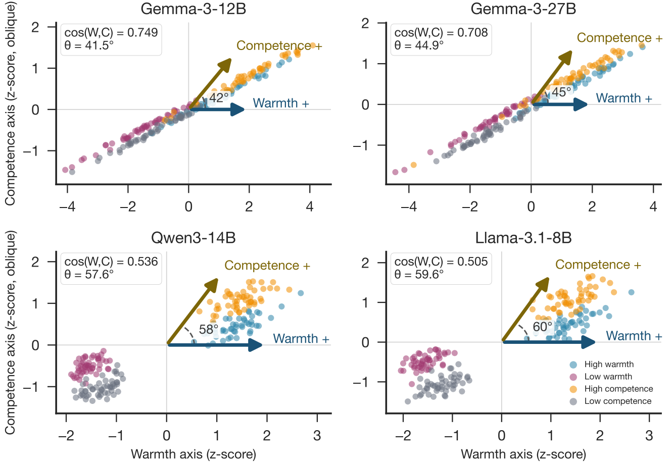
Figure S.1: Conceptual overview. The two dimensions of the Stereotype Content Model (warmth, competence) as encoded in the residual stream of the probed language models. Direction vectors are constructed as mean-difference contrasts between high- and low-condition activations; arrows indicate the positive pole of each axis in the model’s internal representation space.
