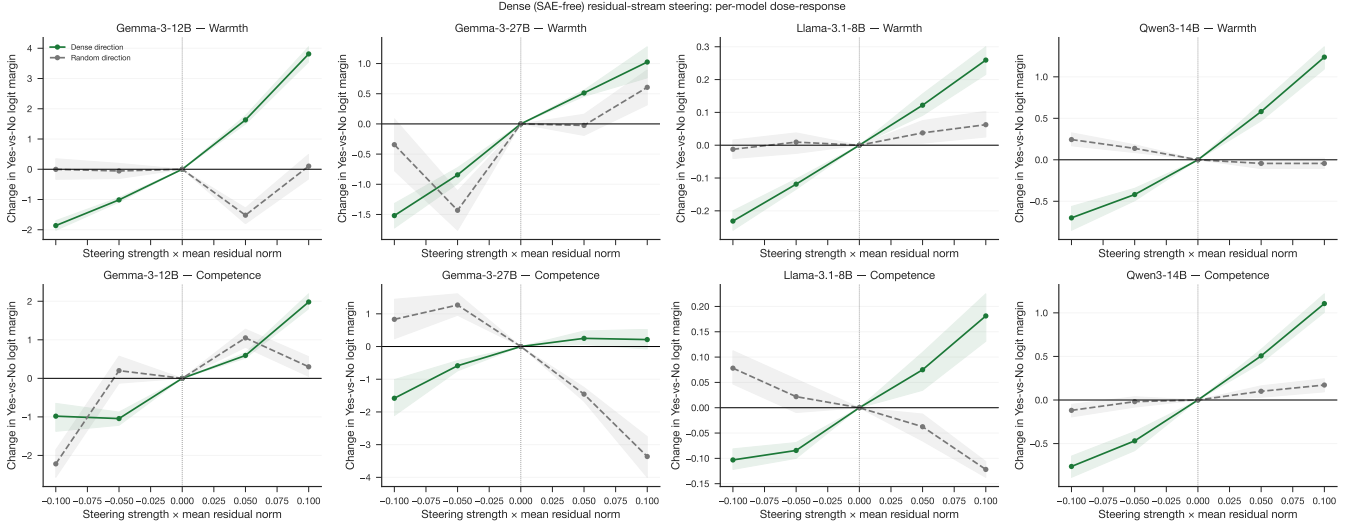
Figure 5: Concept-level steering dose-response curves. Mean logit-margin shift (Yes–No on warmth/competence judgements) as a function of steering strength \alpha (expressed as a fraction of the mean residual-stream norm) for the dense target direction across all four models. Positive slopes confirm that all models respond causally to the extracted direction vectors; the substantially higher slope at Gemma-3-12B (warmth slope = 27.79, R^2 = 0.956 ) compared to Gemma-3-27B (slope = 12.89, R^2 = 0.990 ) illustrates the steerability difference despite identical probe accuracy. Error bars are bootstrapped 95% confidence intervals over held-out topics.
