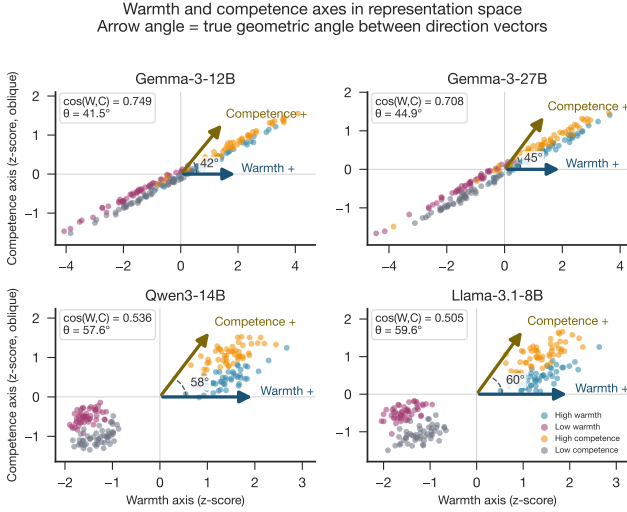
Figure 1: Conceptual overview. The two dimensions of the Stereotype Content Model (warmth, competence) as encoded in the residual stream of the probed language models. Direction vectors are constructed as mean-difference contrasts between high- and low-condition activations; arrows indicate the positive pole of each axis in the model’s internal representation space.
