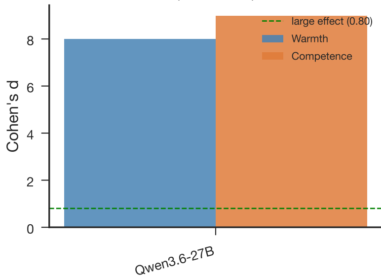
Effect size (Cohen's d)
