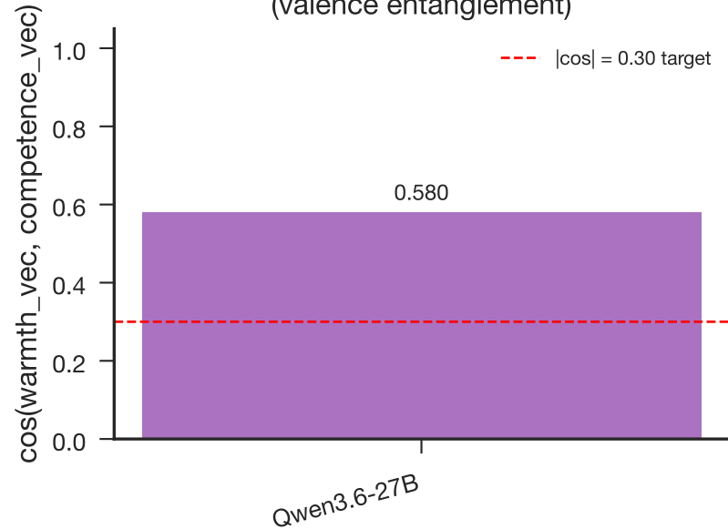
Axis geometric overlap (valence entanglement)
