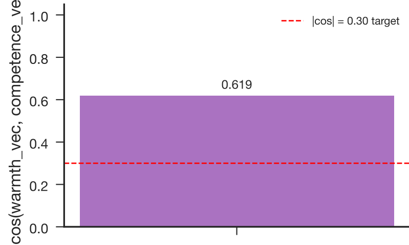
Axis geometric overlap (valence entanglement)
