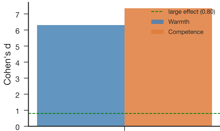
Effect size (Cohen's d)
