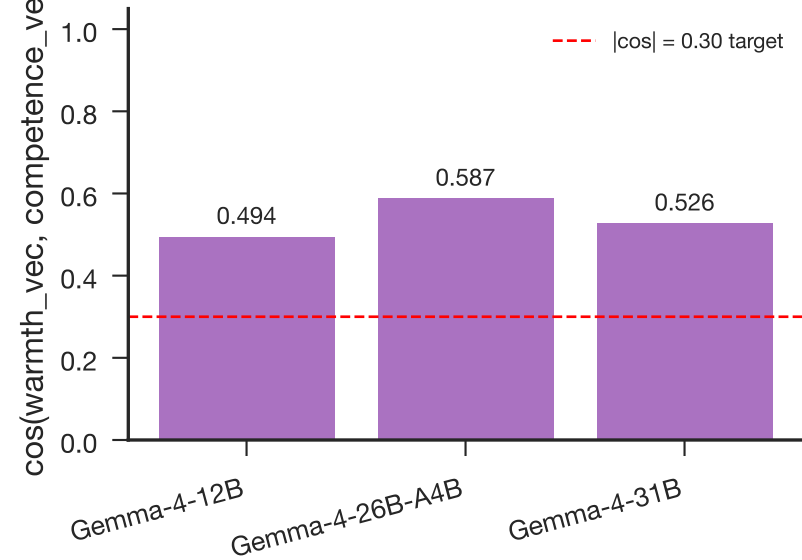
Axis geometric overlap (valence entanglement)
