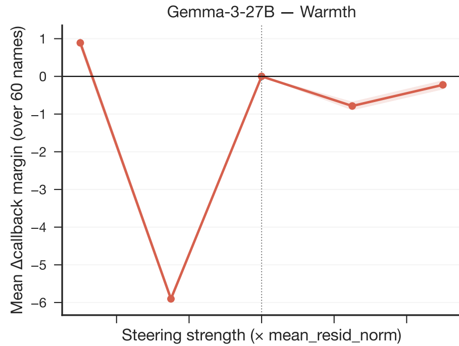
Steering \square callback: mean \Delta margin over 60 names \pm 95% CI (name-level)
