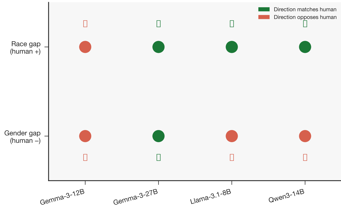
(B) Direction agreement with human benchmark
