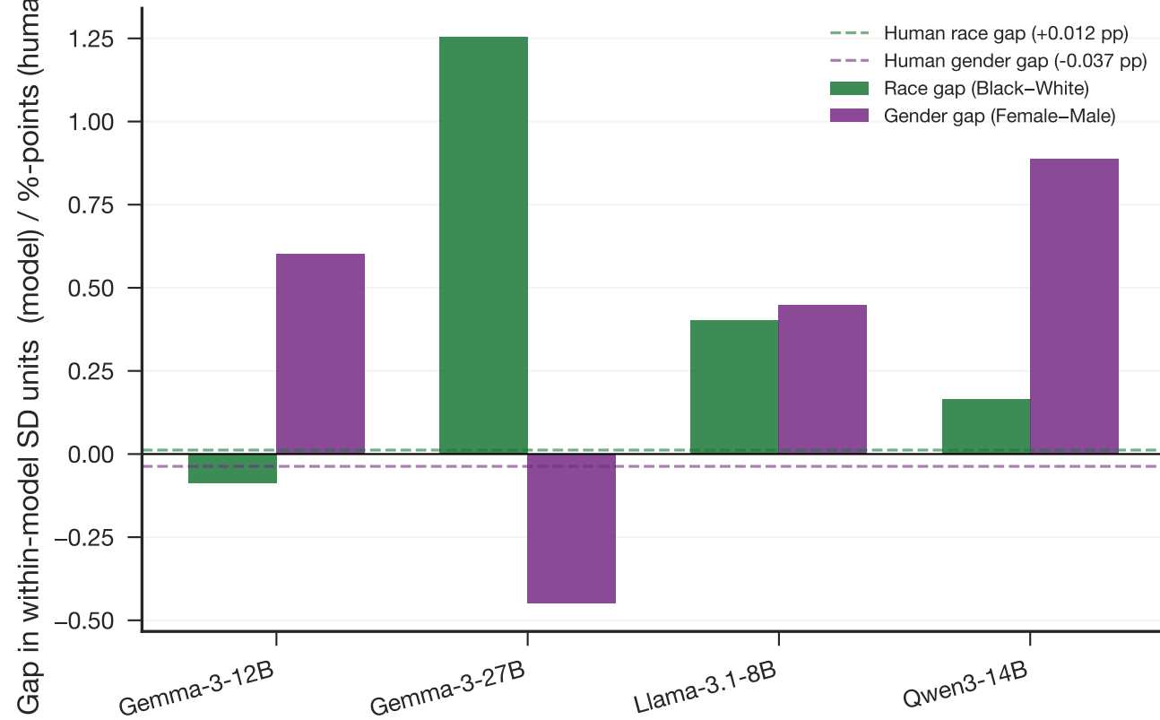
(A) Disparity magnitude — model gaps in within-model SD units
