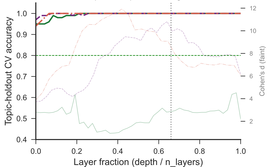
Competence probe emergence
