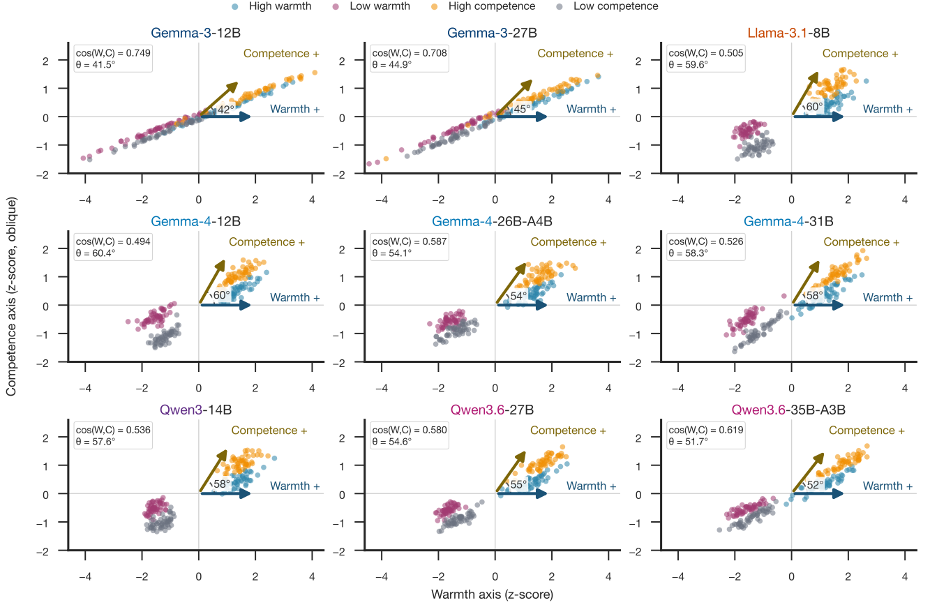
Figure 4: Warmth and competence directions share model-dependent geometry. Each panel projects the same 200 synthetic stories onto raw dense probe-layer directions in an oblique basis. The arrow angle equals \arccos[\cos(v_W, v_C)] , so smaller angles indicate stronger geometric alignment. All panels use model-internal z-scores, shared axis limits, and equal x/y scaling.
