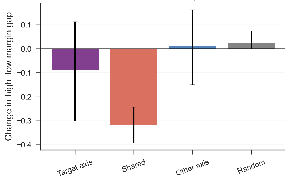
Gemma-3-27B — Competence
