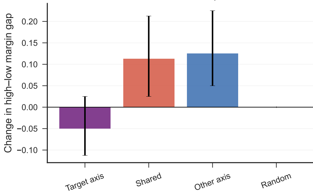
Gemma-3-12B — Competence
