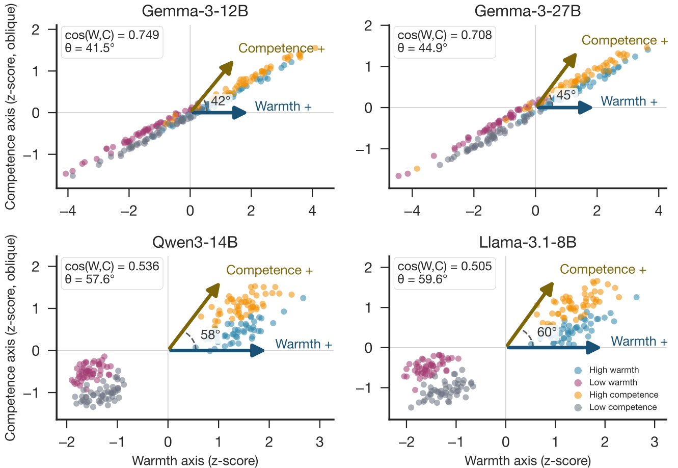
Figure 3: Warmth and competence directions share model-dependent geometry. Each panel projects the same 200 synthetic stories onto raw dense probe-layer directions in an oblique basis. The arrow angle equals \arccos[\cos(v_W, v_C)] , so smaller angles indicate stronger geometric alignment. All panels use model-internal z-scores, shared axis limits, and equal x/y scaling.
