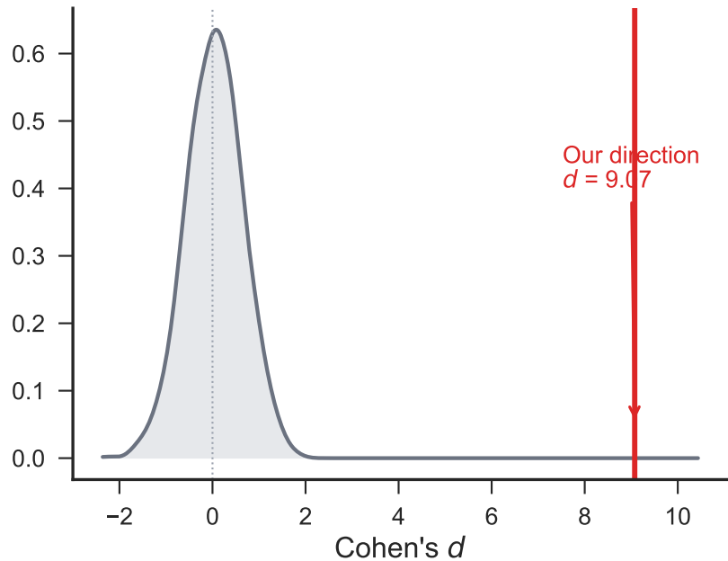
Null distribution — competence axis
