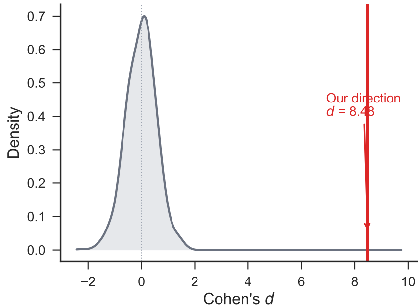
Null distribution — warmth axis
