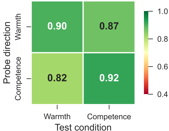
Behavioural discriminability (5-fold CV accuracy, 1-D projection)
