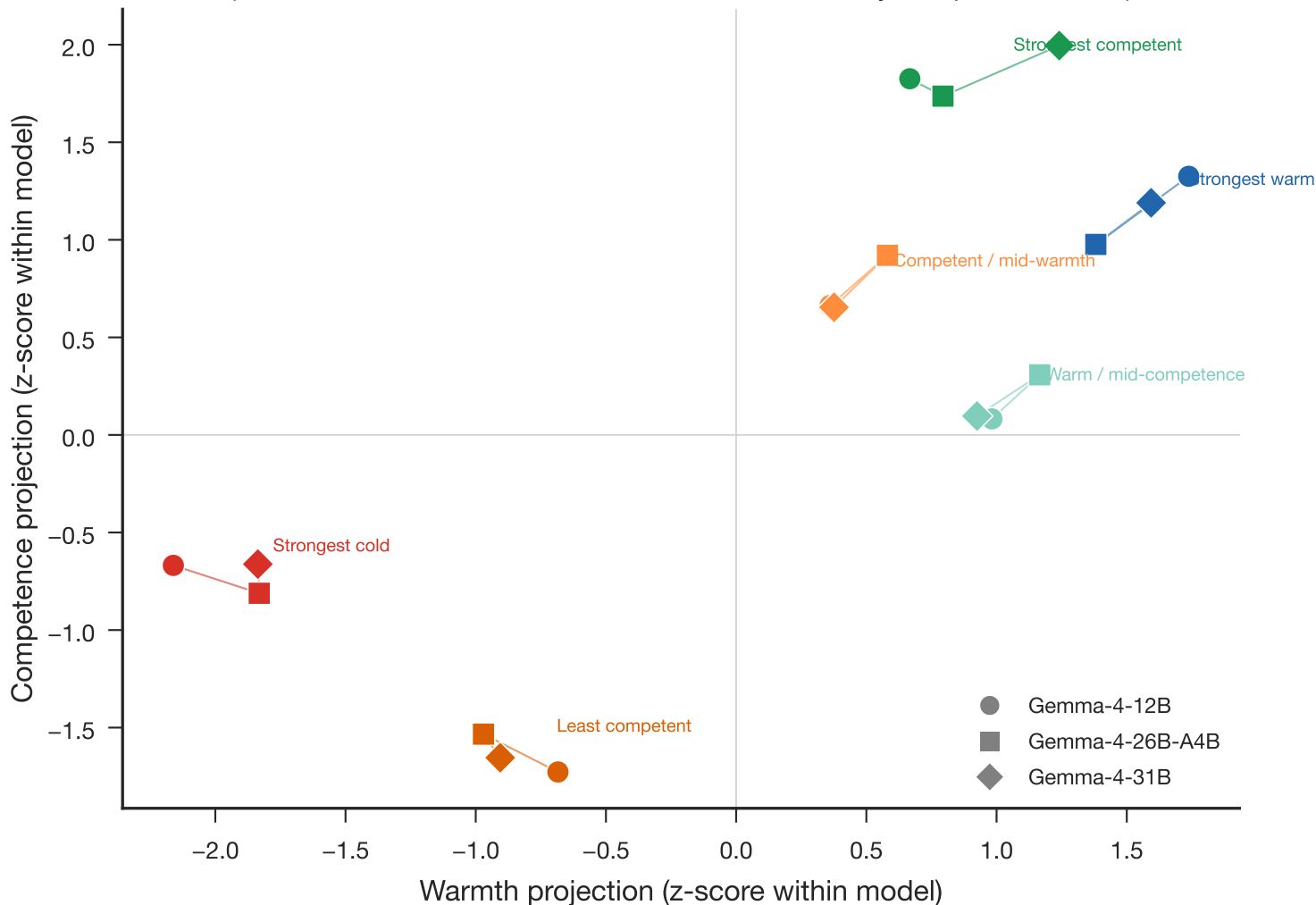
Six Gemma-4-12B-selected exemplar stories across three models (Qualitative illustration; lines connect the same story; shapes = models)
