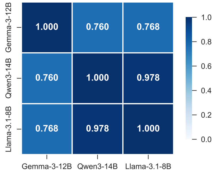
Warmth projection (Spearman \rho , 200 stories)
