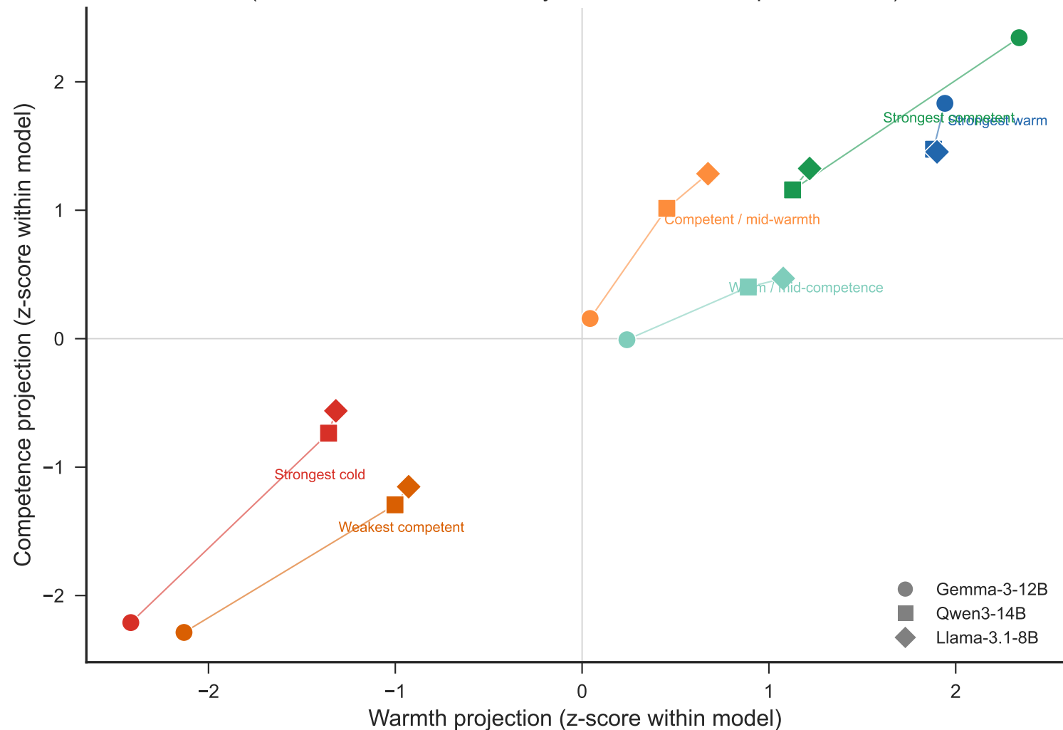
Same stories, three models: convergent placement (Lines connect the same story across models; shapes = models)
