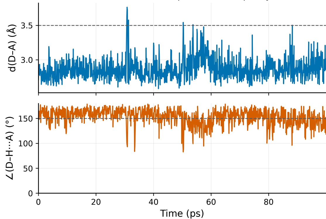
WAT24244 O-HH12 ... Asp16 O — occupancy 64.1%
