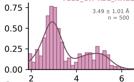
Y115_OH-R32_HH11
